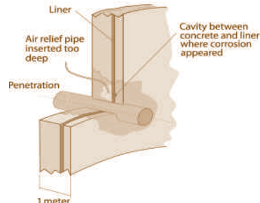
Schematic drawing of containment, Forsmark unit 1 and 2.
