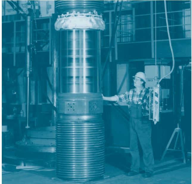
Emergency cooling testing - Simulation of extreme conditions in a feedwater line
