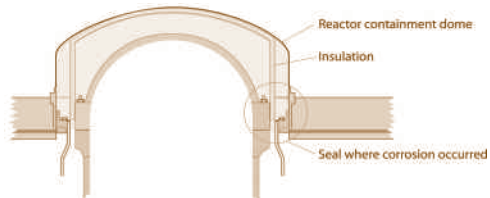
Corrosion attack at the seal connecting liner and the containment cupola, Forsmark unit 1.
